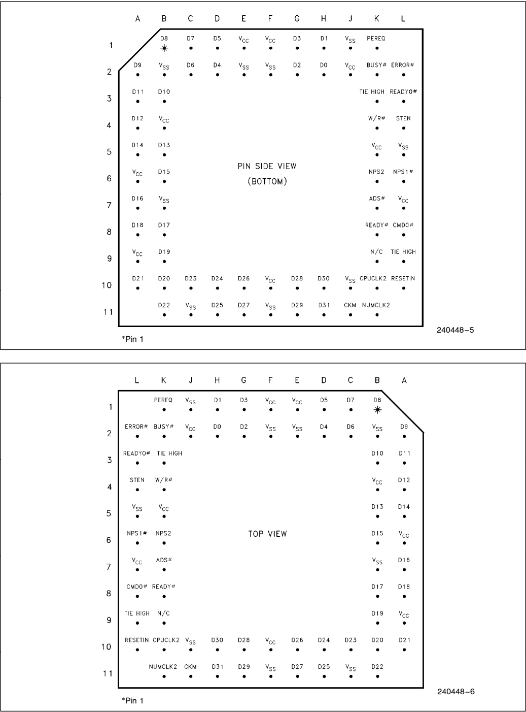
Figure 3.1. Intel387™ DX MCP Pin Configuration
