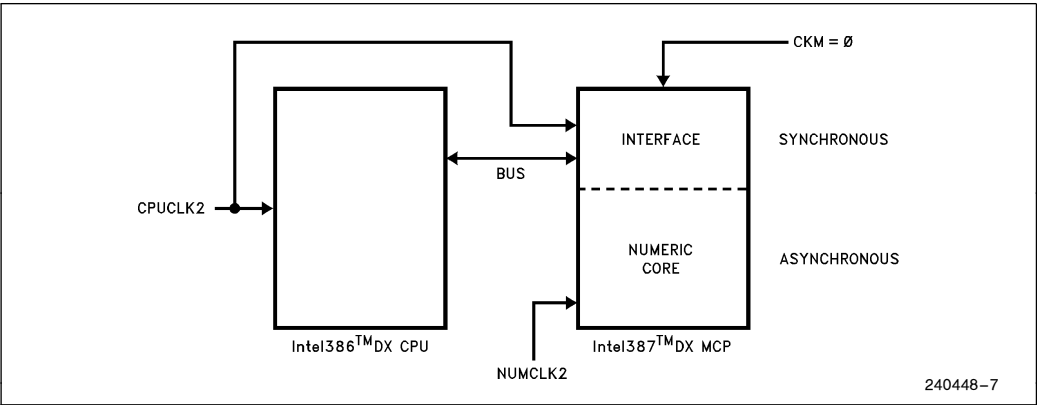
Figure 3.2. Asynchronous Operation
