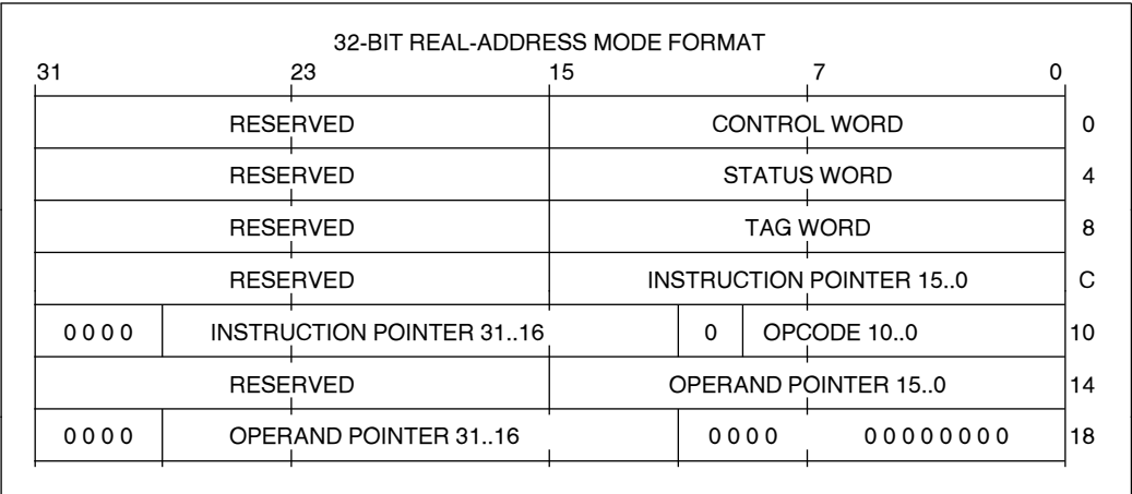
Figure 2.4. Real Mode Intel387™ DX MCP Instruction and Data Pointer Image in Memory, 32-Bit Format
